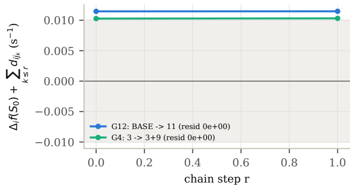
Chain identity: no sign crossing along nested chains
