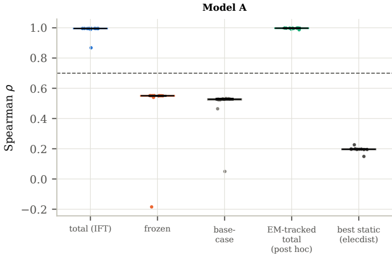
Spearman correlation with the finite x1.5 branch effect (12 holdout conditions per model; dashed: gate 0.70)
