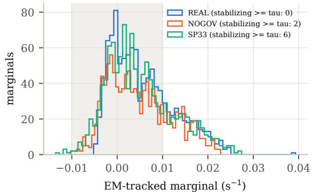
EM-tracked marginals: almost only destabilizing
