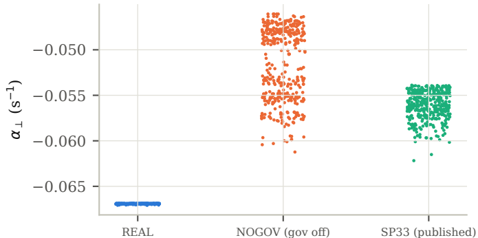
Rightmost transverse eigenvalue: slow real poles in every variant
