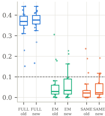
material regret rate
