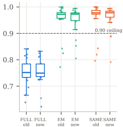
optimal fixed-ranking agreement p^*
