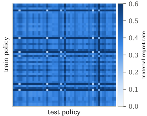
regret of ranking fitted at row policy, used at column policy
