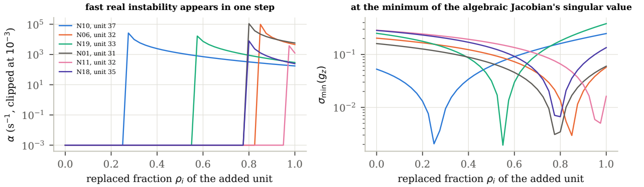
Figure S6: Fractional-replacement sweeps: \alpha_{\perp} and the minimum singular value of g_z against the replaced fraction.
