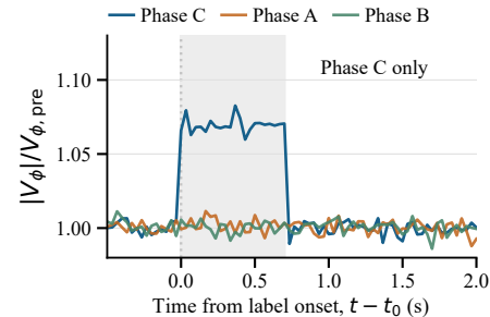
(f) Corrupted voltage at PMU 2
