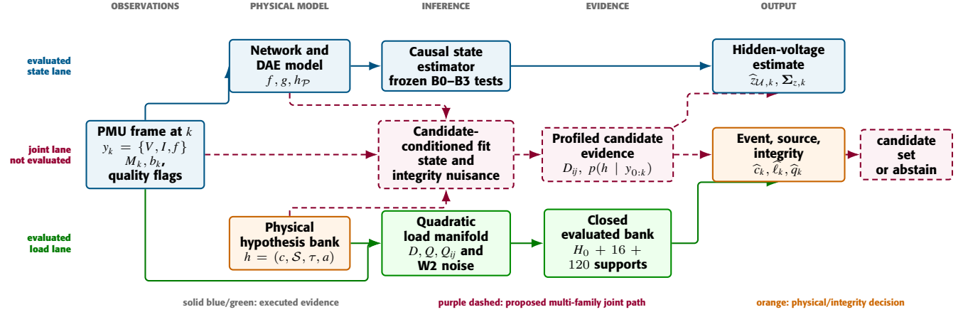
FIGURE 1. Scientific argument and validation boundary. The blue B0–B3 path is an independently evaluated state-reconstruction component. The green path is the implemented batch reference estimator \mathcal{E}_B . The dashed path is the proposed joint estimator \mathcal{E}_j ; its complete posterior remains unevaluated. The exploratory single-event pilot implements only part of that route.
