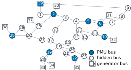
(a) IEEE 39-bus sensing geometry
