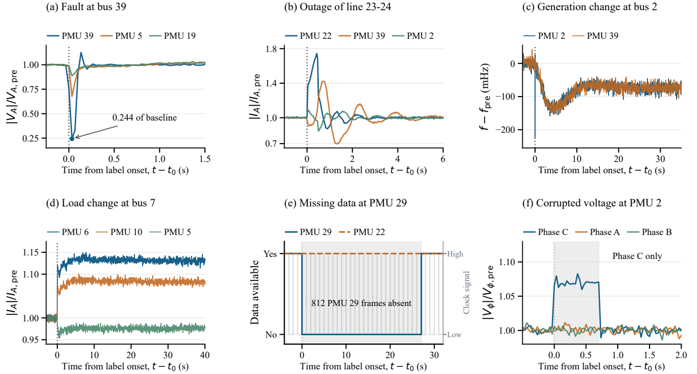
FIGURE 4. Representative measured signatures from the RAW0001 reference simulation. Physical events alter voltage, current, or frequency through the network; integrity events alter availability or channel consistency. In panel (e), the gray reference clock advances while PMU 29 packets are absent. Curves are unsmoothed, and each panel uses the time scale needed to show its physical response.
