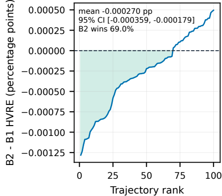
(c) Paired temporal contribution
