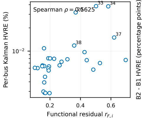
(b) Structure predicts difficulty
