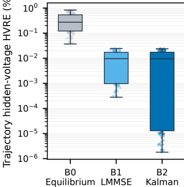
(a) Frozen nominal TEST distributions
