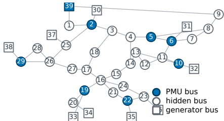
(a) IEEE 39-bus sensing geometry
