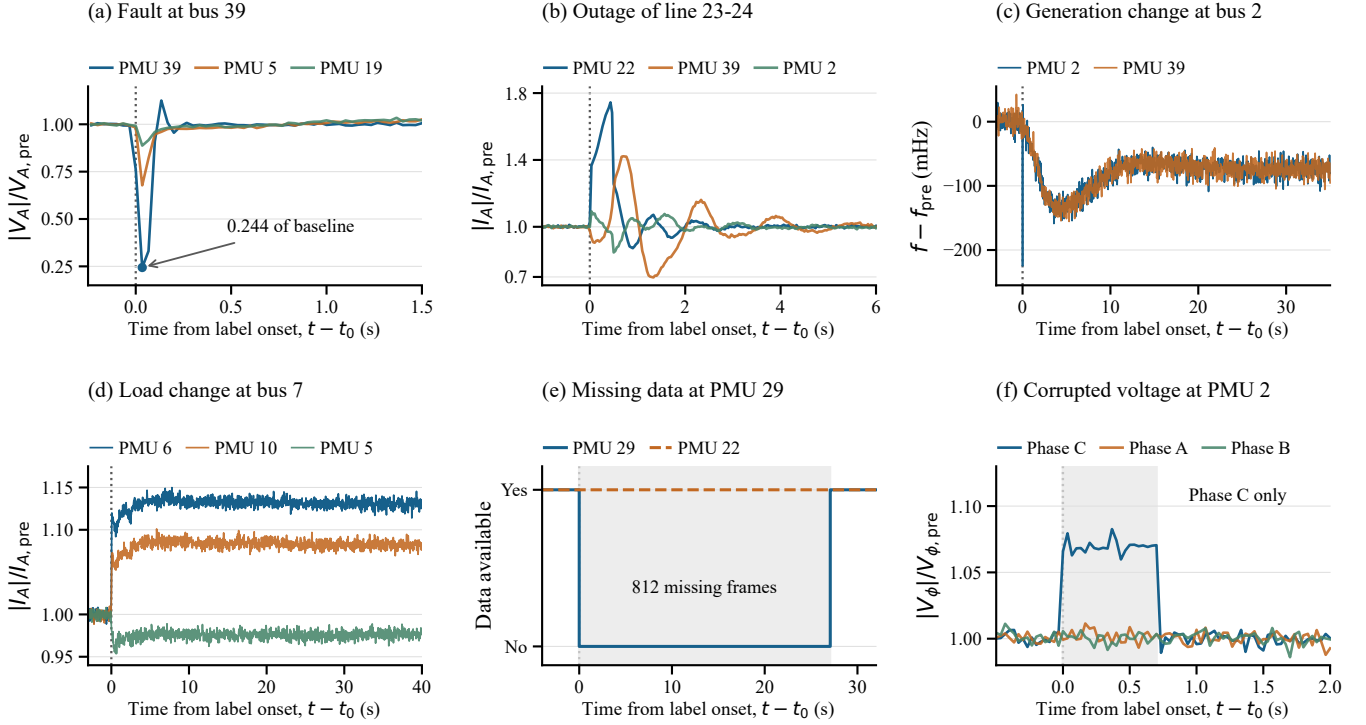
FIGURE 5. Representative measured event signatures from RAW0001, sampled at approximately 30 frames/s. (a) Bus fault, (b) line outage, (c) generation change, (d) load change, (e) missing data, and (f) single-phase corruption. The 812-frame missing interval in (e) is approximately 27.1 s. Dotted lines mark the first labeled sample; gray shading marks missing or corrupted intervals. Magnitudes are normalized by the preceding 3-s median, frequency is relative to its corresponding median, and time scales differ by panel. The plotted values and source-file hashes are frozen in the evidence snapshot.
