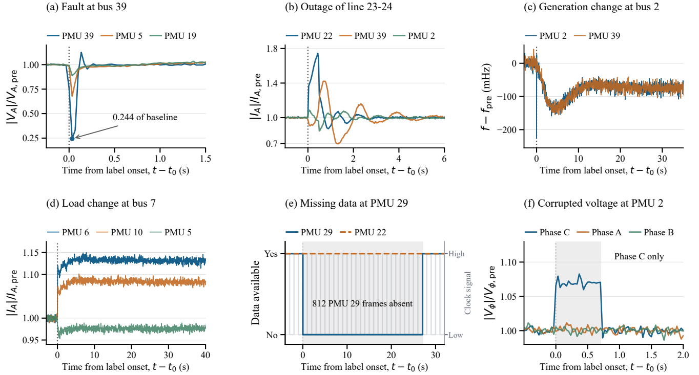
FIGURE 4. Representative measured signatures from the RAW001 reference simulation. Physical events alter voltage, current, or frequency through the network; integrity events alter availability or channel consistency. In panel (e), the gray reference clock advances while PMU 29 packets are absent. Curves are unsmoothed, and each panel uses the time scale needed to show its physical response.
