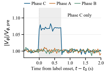
(f) Corrupted voltage at PMU 2
