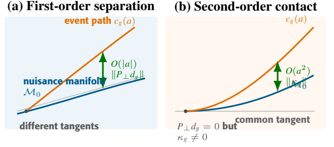
FIGURE 4. Local diagnosability after whitening. (a) A projected event tangent gives first-order separation. (b) Nuisance absorbs the tangent, but relative curvature yields squared separation proportional to a^4 . Event curvature alone is insufficient because the nuisance manifold can bend with it.
