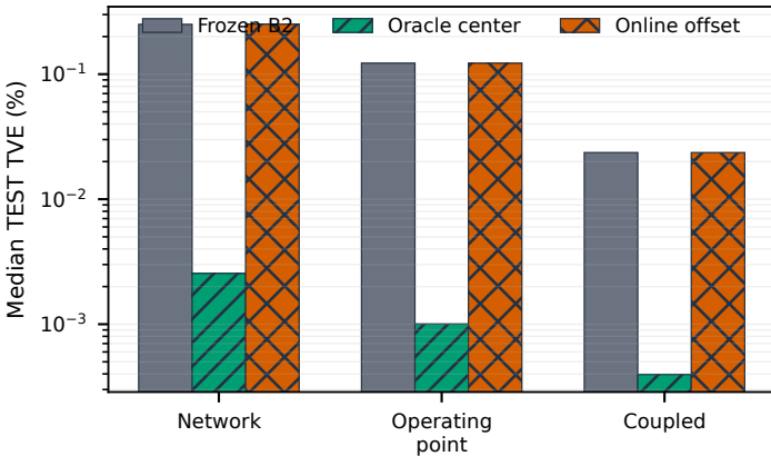
(a) Causal offset proxy does not close oracle gap
