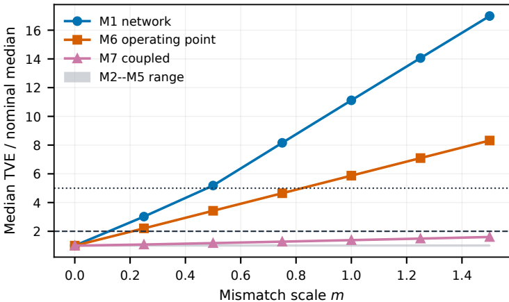
(a) Frozen Kalman estimator under rebuilt plants
