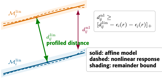
FIGURE 4. Local source-diagnosability geometry. State and integrity nuisance generate one affine response set per candidate. The shortest weighted separation determines the linear margin. The shaded tubes represent bounded nonlinear remainders; overlap can erase a positive linear margin.
