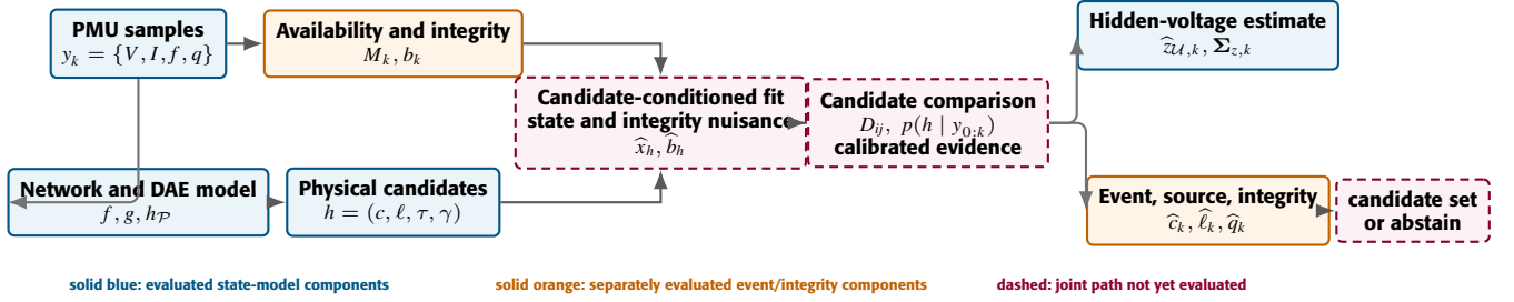
FIGURE 1. Inference path and validation boundary. PMU samples and quality flags enter candidate-specific DAE simulation and nuisance fitting. The fitted candidates produce a state estimate and an event, source, and integrity decision with optional abstention. Solid boxes denote evaluated components; dashed boxes denote the end-to-end candidate comparison that still requires a common experiment.
