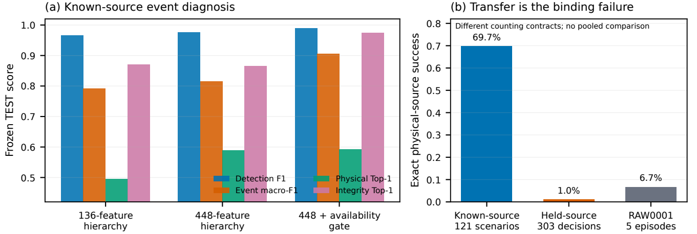
FIGURE 10. Event evidence and its transfer boundary. (a) Known-source TEST metrics for the compact hierarchy, expanded hierarchy, and availability-gated model. (b) Exact physical-source success under three distinct counting protocols: known-source completed scenarios, source-held-out decisions, and RAW0001 physical episodes. The bars in (b) are deliberately not pooled; they expose the change in task difficulty and data semantics.
