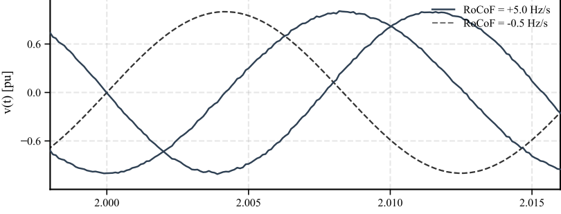
Group G2 (E8 → E9) Frequency Ramps — Voltage (G2-E8 / G2-E9)
