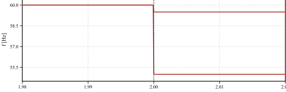
Group G2 (E7 → E6) Frequency Steps — Frequency (G2-E7 / G2-E6)
