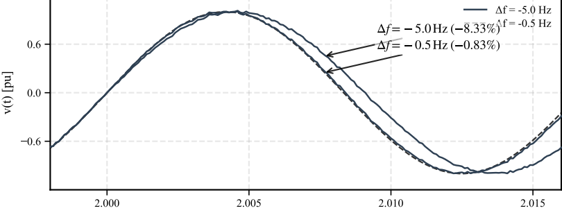
Group G2 (E7 → E6) Frequency Steps — Voltage (G2-E7 / G2-E6)
