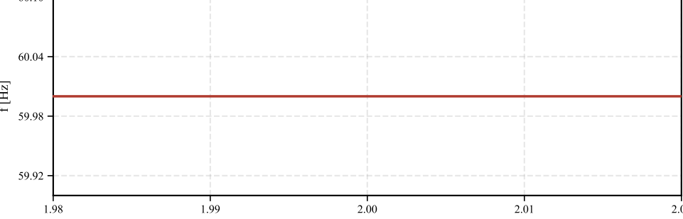
Group G2 (E5 → E4) Voltage Steps — Frequency (G2-E5 / G2-E4)
