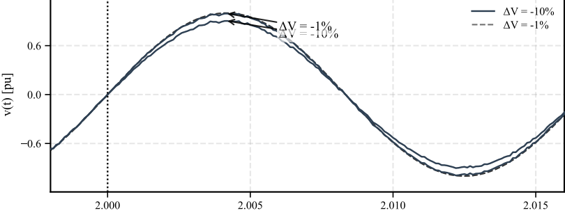
Group G2 (E5 → E4) Voltage Steps — Voltage (G2-E5 / G2-E4)
