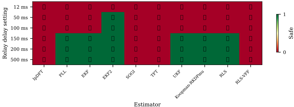
A4: Relay coordination safety (green=safe, red=trips)
