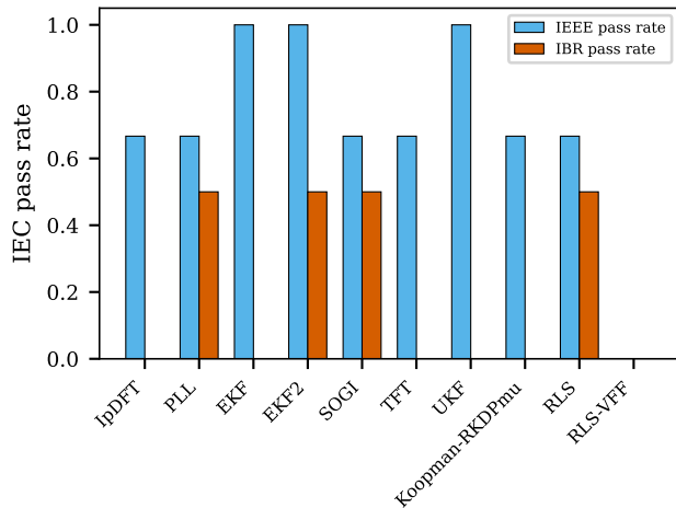
IEC pass rate: IEEE vs IBR scenarios
