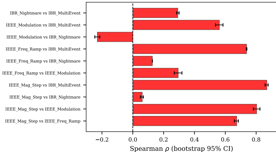
B3: Scenario rank correlation with bootstrap CIs
