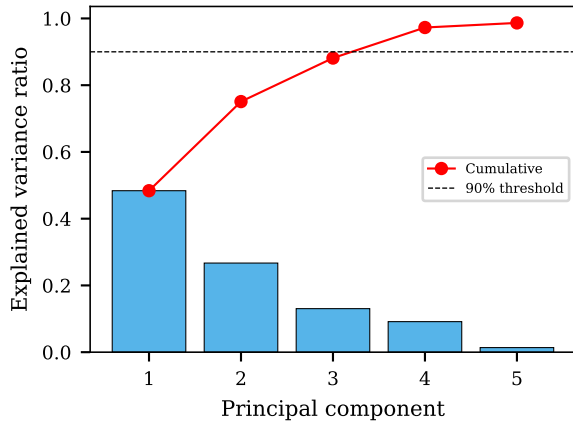
PCA scree plot (90% var in 4 PCs)
