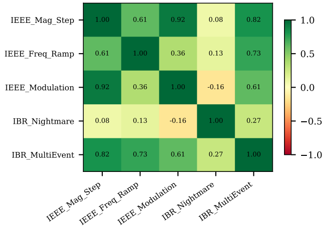
Q6: Scenario Spearman rank correlation
