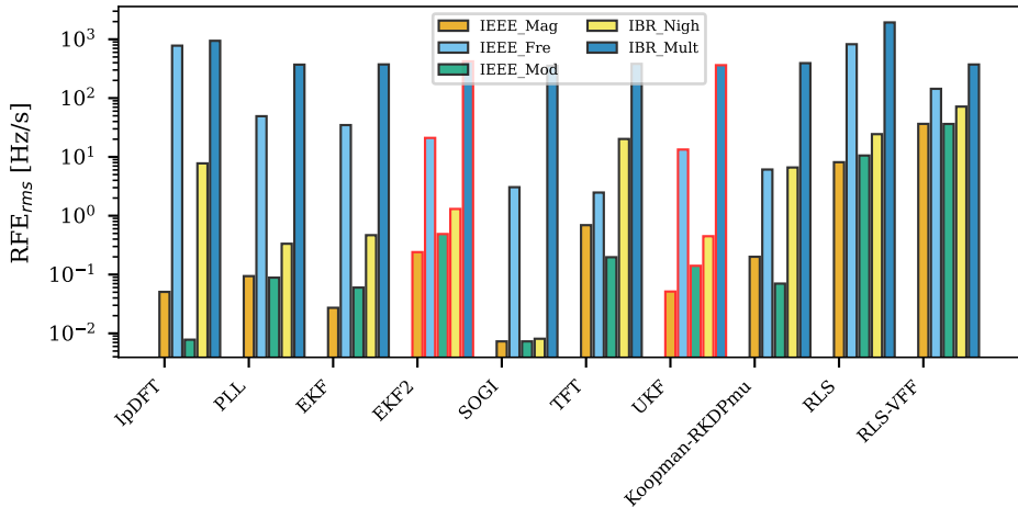
A3: RoCoF estimation error (red border=explicit \dot{\omega} state)
