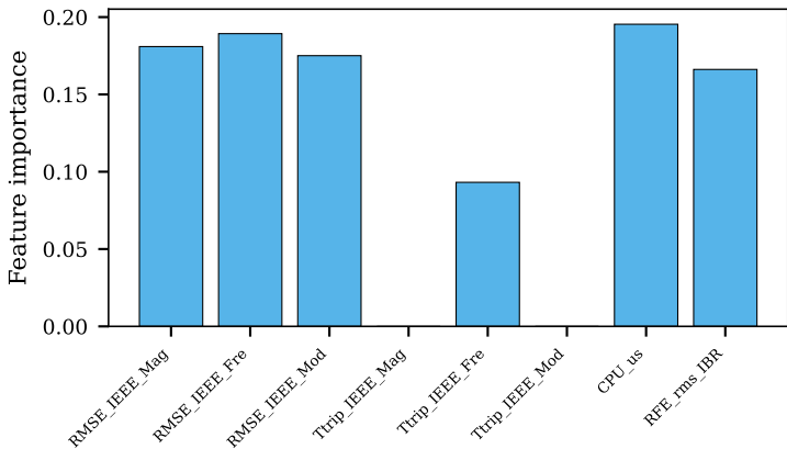
D1: Method selector RF CV acc=1.00
