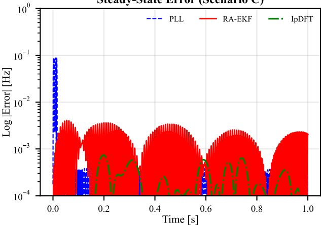
Steady-State Error (Scenario C)
