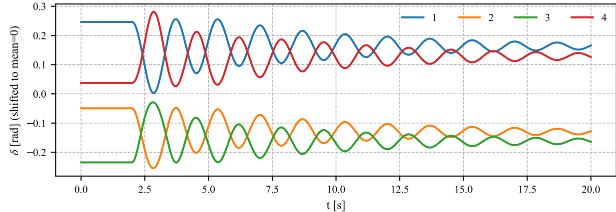
Kundur (ANDES): rotor angle states
