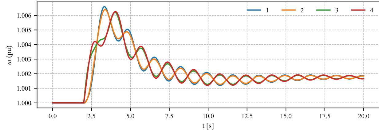
Kundur (ANDES): rotor speed states
