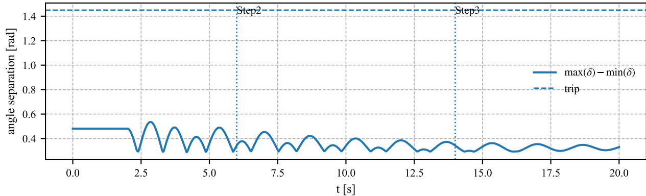
no_fix: Loss-of-synchronism proxy
