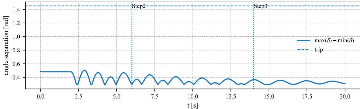
with_fix: Loss-of-synchronism proxy
