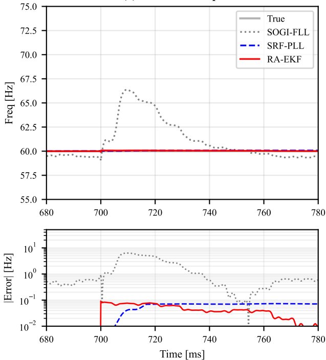
(a) Transient Response
