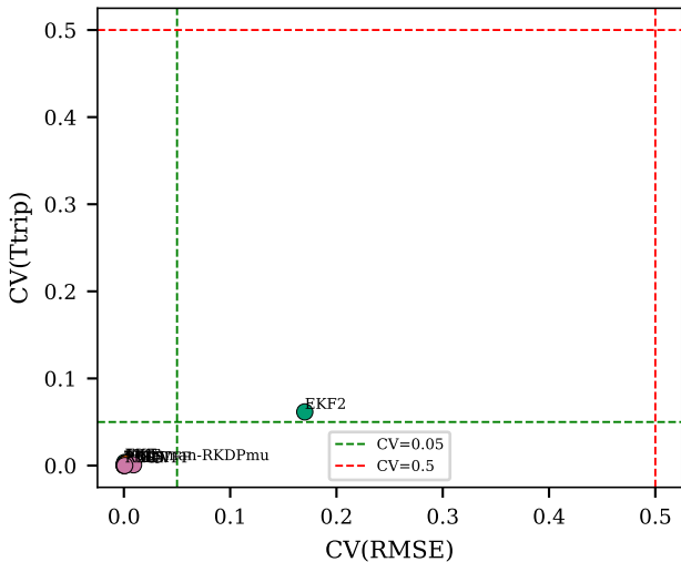
B2: Stochastic vs deterministic metrics
