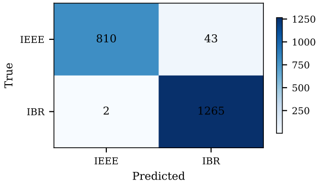
Confusion matrix (training)
