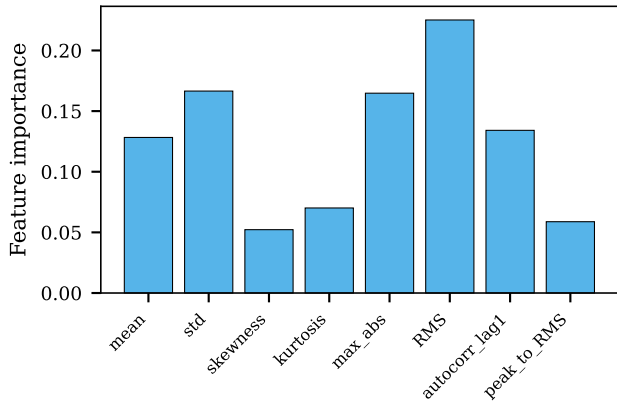
Q4: RF feature importance ACC=0.95±0.02
