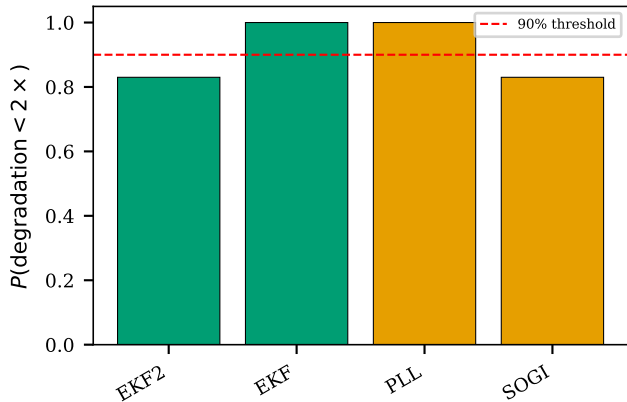
G1: Tuning robustness score
