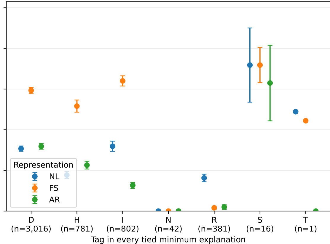
OEQA
