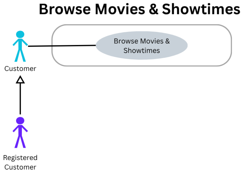
Figure 2. Browse Movies & Showtimes Use Case Diagram
