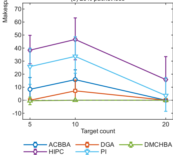
(b) 25% packet loss
