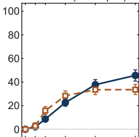
MiniMax (makespan)
