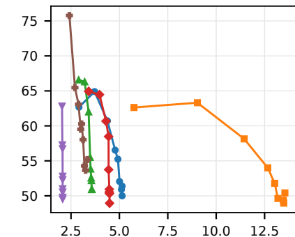
Rayleigh-style
