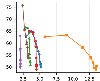
Rayleigh-style
