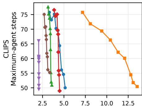
Bernoulli
