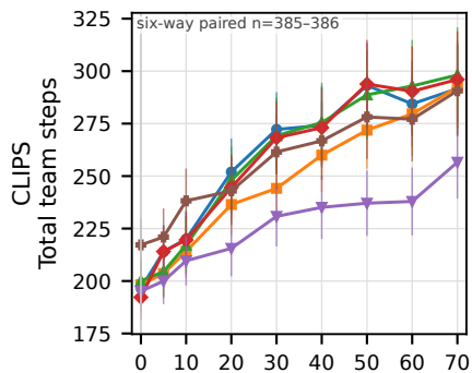
Bernoulli
