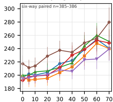
Rayleigh-style
