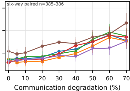
Rayleigh-style
