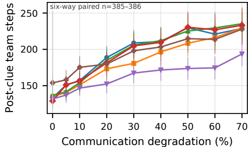
Bernoulli
