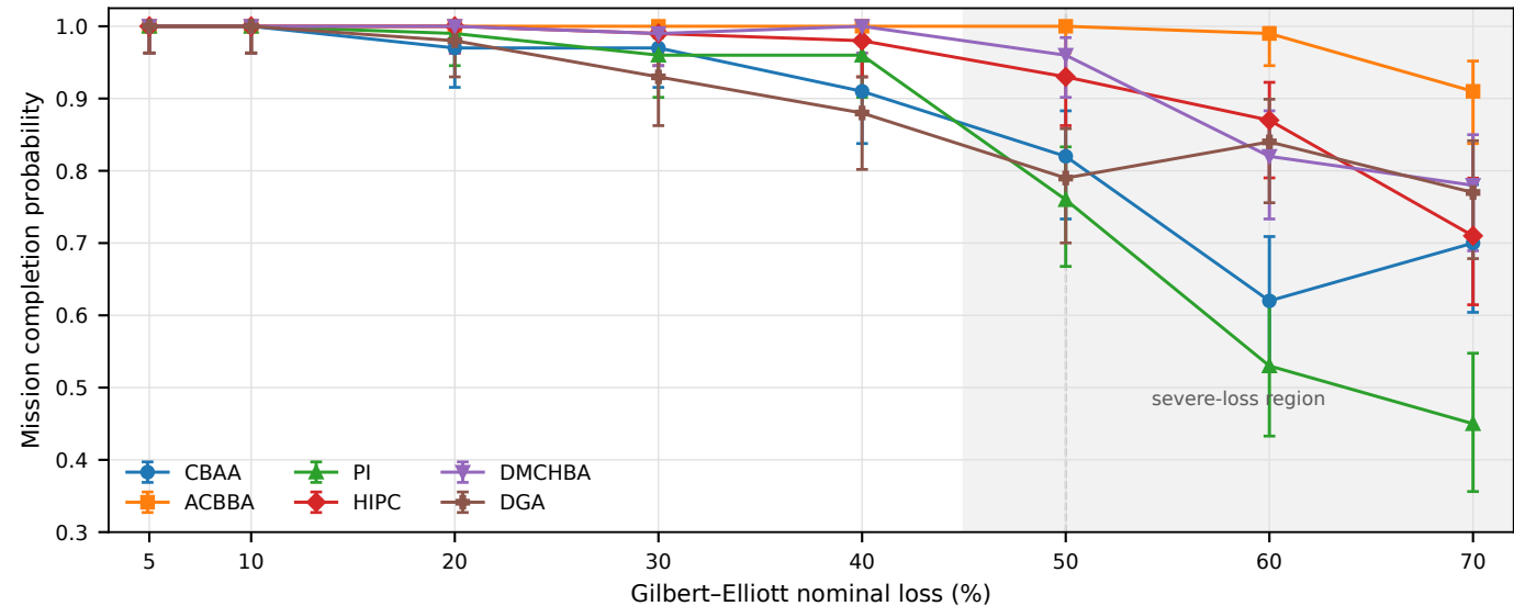
FGS completion reliability (100 matched trials per algorithm and level)
