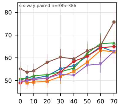
Rayleigh-style
