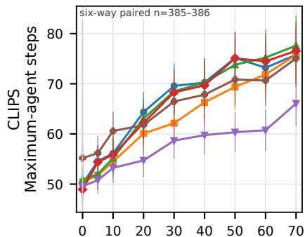
Bernoulli
