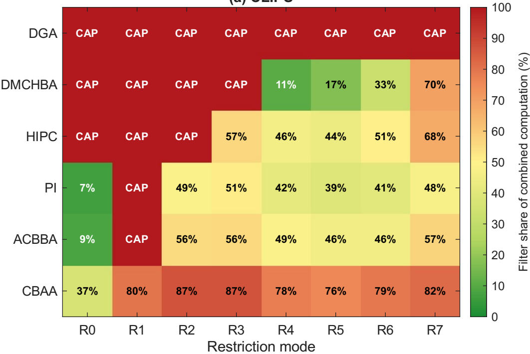
(a) CLIPS
