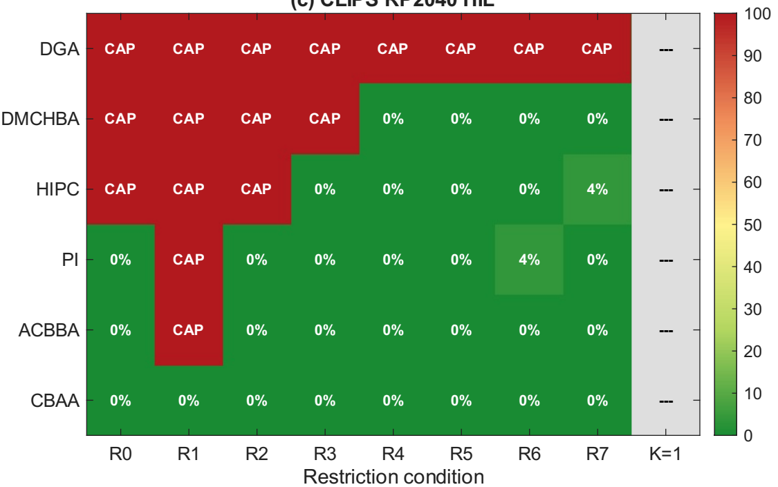
(c) CLIPS RP2040 HIL
