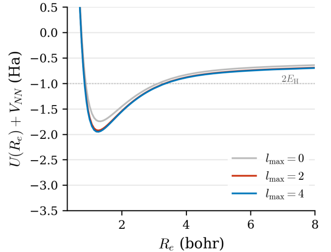
FIG. 3. Adiabatic potential U(R_e) + V_{NN} at R = 1.4 bohr for l_{\max} = 0 (gray), 2 (red), and 4 (blue). The well deepens with increasing l_{\max} as quadrupolar and higher nuclear coupling channels open. The dotted line marks the dissociation threshold 2E_H = -1 Ha.
