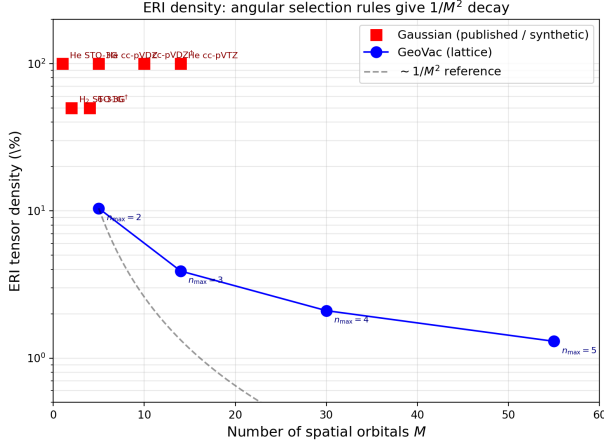
FIG. 2. ERI tensor density versus number of spatial orbitals M . Red squares: Gaussian bases (50–100% dense). Blue circles: GeoVac lattice, showing monotonic decay from 10.4% ( M = 5 ) to 1.3% ( M = 55 ). Gray dashed curve: \sim 1/M^2 reference, normalized to the n_{\max} = 2 data point. The GeoVac ERI density decays as \sim 1/M (empirically \approx M^{-0.85} - M^{-1} ), shallower than the 1/M^2 reference, the decay being imposed by angular momentum selection rules.
