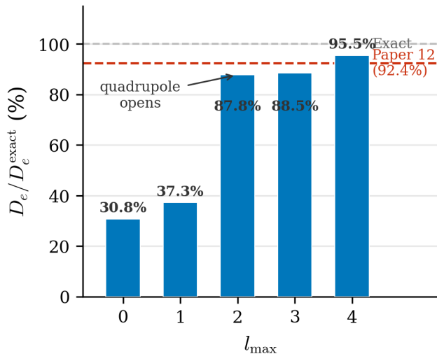
FIG. 2. Percentage of exact dissociation energy recovered as a function of l_{\text{max}} . The dashed line marks Paper 12's 92.4%. The dramatic jump at l_{\text{max}} = 2 reflects the onset of quadrupolar nuclear coupling (Sec. V).
