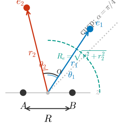
FIG. 1. Molecule-frame hyperspherical coordinates for H_2 . Two nuclei A, B separated by R define the body-frame z -axis. Electrons at \mathbf{r}_1, \mathbf{r}_2 from the midpoint are parameterized by hyperradius R_e = \sqrt{r_1^2 + r_2^2} , correlation angle \alpha = \arctan(r_2/r_1) , and polar angles \theta_1, \theta_2 from the inter-nuclear axis. The cusp locus \alpha = \pi/4 (dotted) is geometry-independent.
