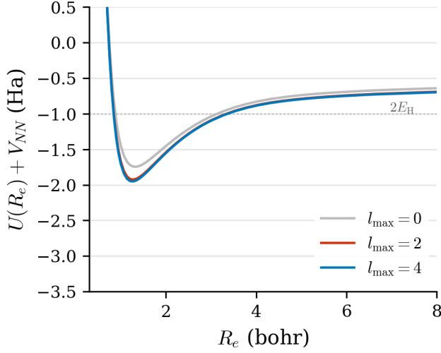
FIG. 3. Adiabatic potential U(R_e) + V_{NN} at R = 1.4 bohr for l_{\max} = 0 (gray), 2 (red), and 4 (blue). The well deepens with increasing l_{\max} as quadrupolar and higher nuclear coupling channels open. The dotted line marks the dissociation threshold 2E_H = -1 Ha.
