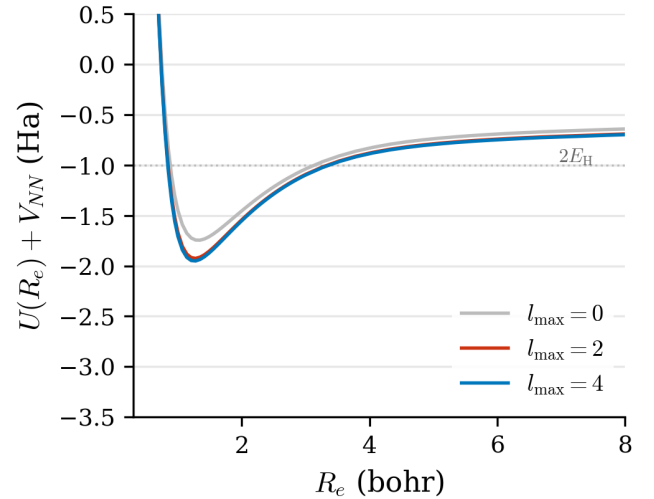
FIG. 3. Adiabatic potential U(R_e) + V_{NN} at R = 1.4 bohr for l_{\max} = 0 (gray), 2 (red), and 4 (blue). The well deepens with increasing l_{\max} as quadrupolar and higher nuclear coupling channels open. The dotted line marks the dissociation threshold 2E_H = -1 Ha.
