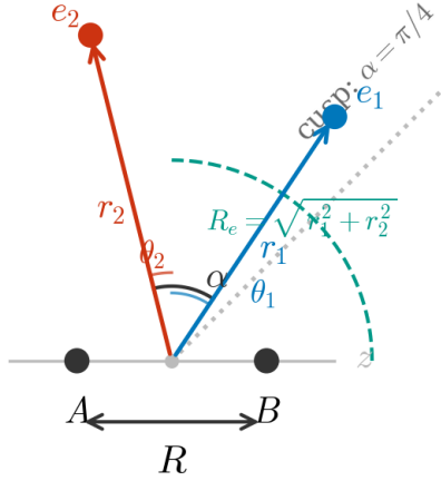
FIG. 1. Molecule-frame hyperspherical coordinates for \text{H}_2 . Two nuclei A, B separated by R define the body-frame z -axis. Electrons at \mathbf{r}_1, \mathbf{r}_2 from the midpoint are parameterized by hyperradius R_e = \sqrt{r_1^2 + r_2^2} , correlation angle \alpha = \arctan(r_2/r_1) , and polar angles \theta_1, \theta_2 from the inter-nuclear axis. The cusp locus \alpha = \pi/4 (dotted) is geometry-independent.
