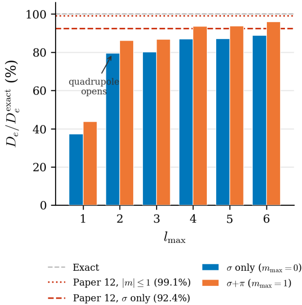
FIG. 2. Percentage of exact dissociation energy recovered as a function of l_{\max} , for both azimuthal sectors. Bars are the \sigma and \sigma+\pi columns of Table II (2D solver with Schwartz cusp correction); the figure is drawn from that table and adds no data of its own. Both Paper 12 reference values are shown and each is labelled with the sector it belongs to: its \sigma -only 92.4% and its |m| \leq 1 99.1%. Neither is a like-for-like reference for these curves—the truncation and the solver class differ—and no ordering between the two coordinate systems is asserted here or anywhere in this paper. The jump at l_{\max} = 2 (+42.3 points, the largest step in the table) reflects the onset of quadrupolar nuclear coupling (Sec. V).
